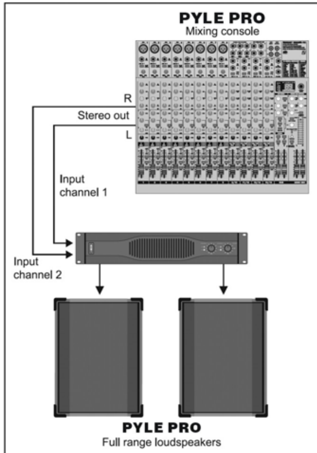
Fig .3.1:2-channel mode
